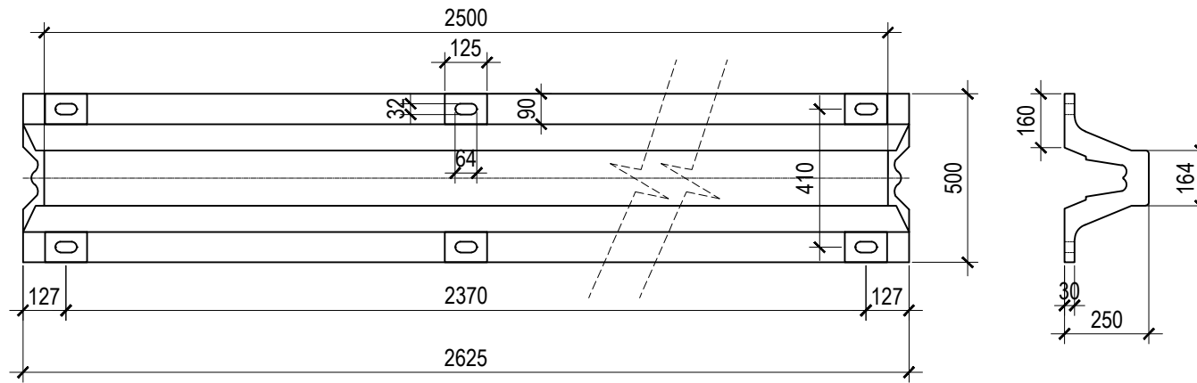
A2 01 TYPICAL DETAIL OF PORT FENDER SCALE
